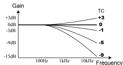
Diagram of Tone Control
