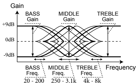
Diagram of 3-bands Equalizer
