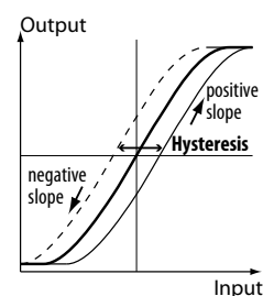
How the Trans - Hysteresis works
